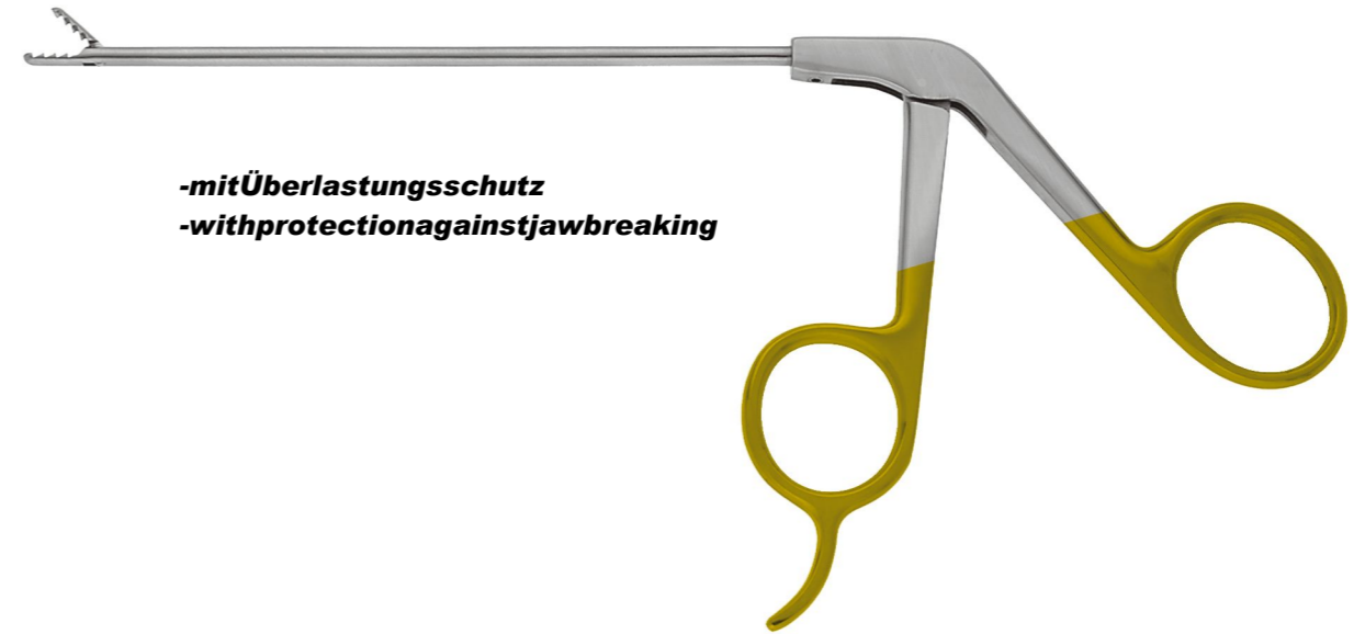
Mikroscherenstanze Micro-Scissors-Punch L=5,0mmB=0,8mm
